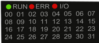
Display block for module BMXDDO6402K
