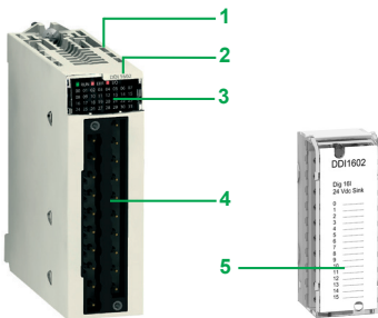
Module for connection via 20-way removable terminal block
