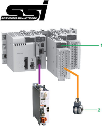
Modicon X80 modules platform with Modicon M340 processor
