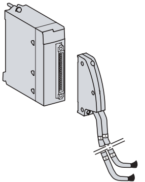
Preformed cordset with 40-way connector at one end and 2 flying leads at the others
