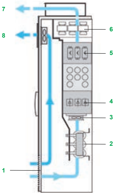
IP23 enclosure
